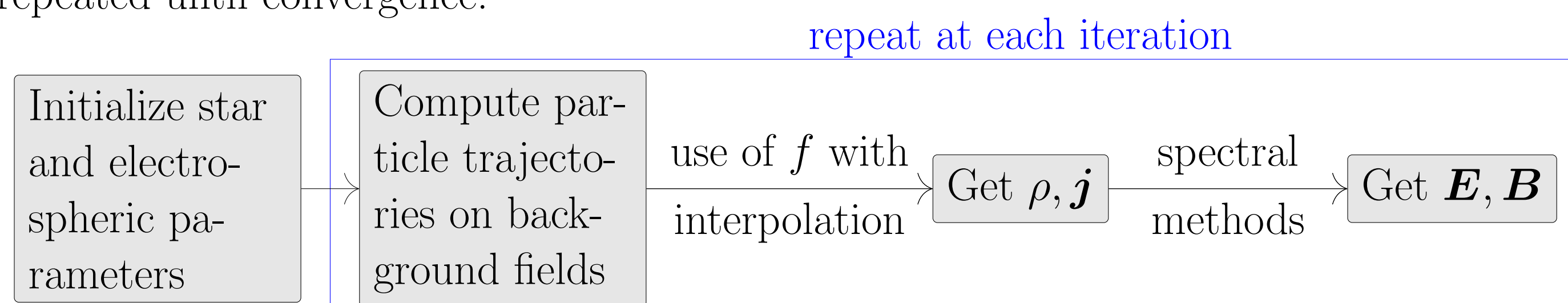
Fig. 1: Iteration scheme to compute a numerical solution of charge and current densities ( \rho, j ) and electromagnetic fields ( E, B ). f is the distribution function of the particles.
